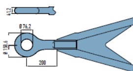
Towing eye type NATO VG-74059 D value = 125 kN
