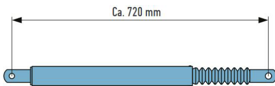
Klemmfix 72/Z effective on tension 51.98.01.0013
