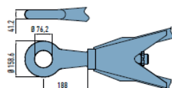
Screw-in towing eyes type NATO VG-74059 D value = 125 kN
