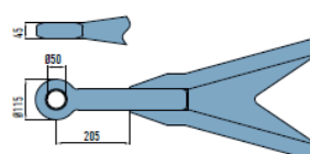
Towing eye VBG 16-0895 D value = 190 kN
