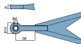
Towing eye: version for Switzerland D value = 168 kN
