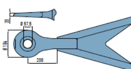
Towing eye VBG 15-173 D value = 190 kN
